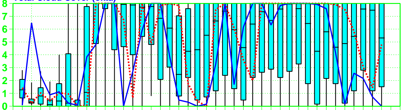
Total Cloud Cover (okta)
